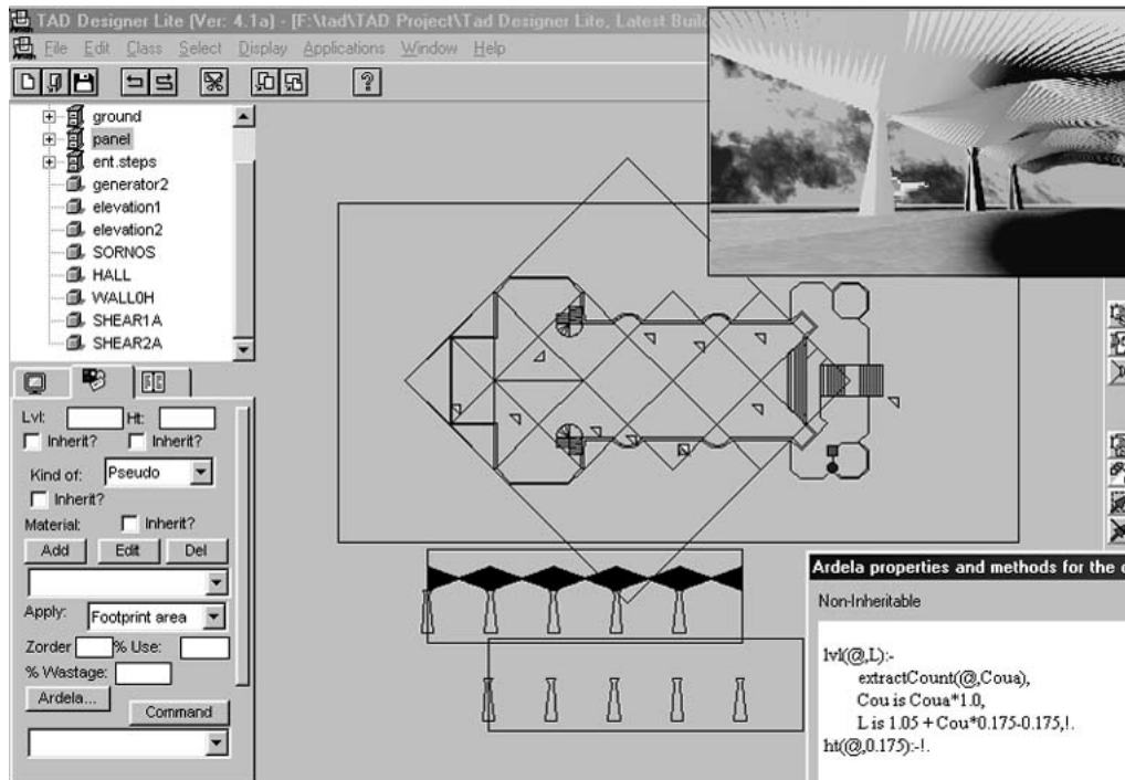
Figure 1 (left). Screenshot of TAD Designer Lite showing the structure of a church, and a rendered image of the church (separately generated) in the top right.
